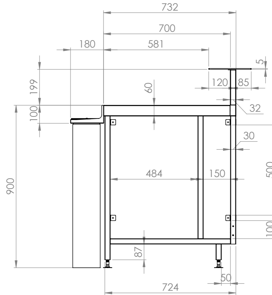
SIDE ELEVATION
