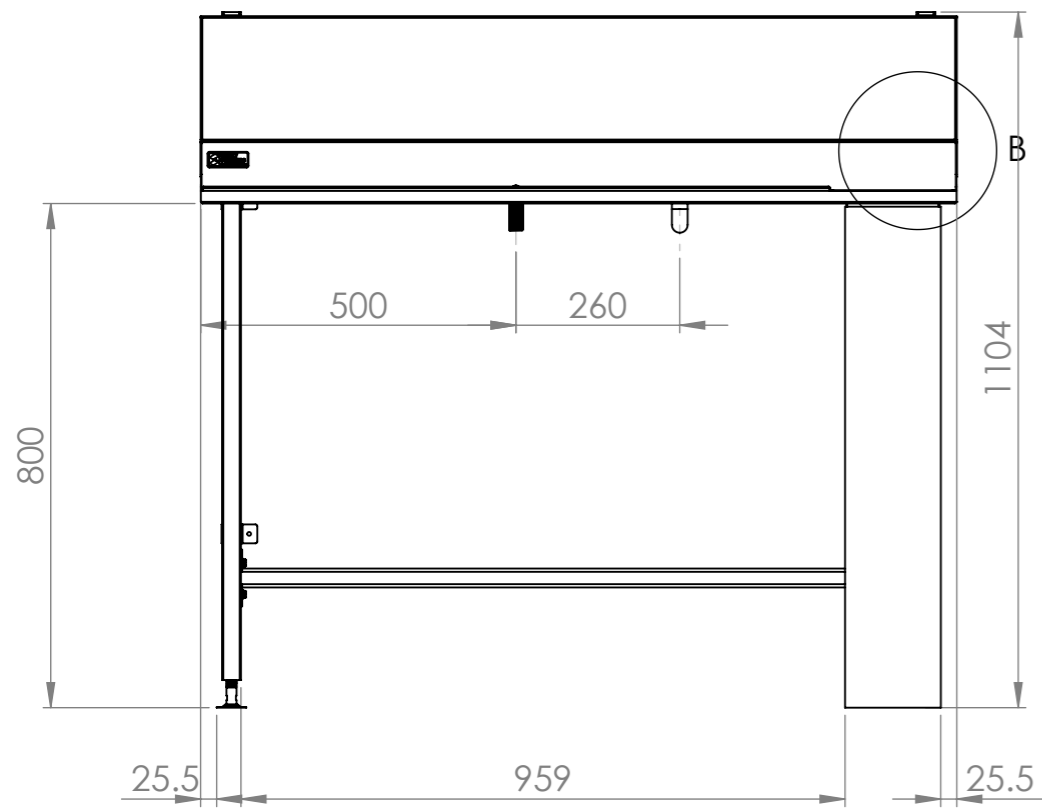
FRONT ELEVATION
