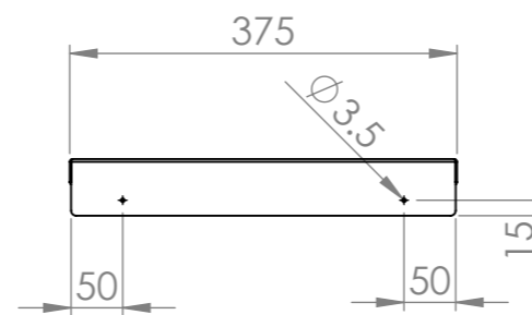
SIDE ELEVATION
