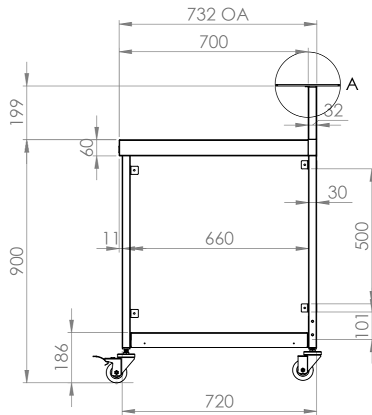
SIDE ELEVATION
