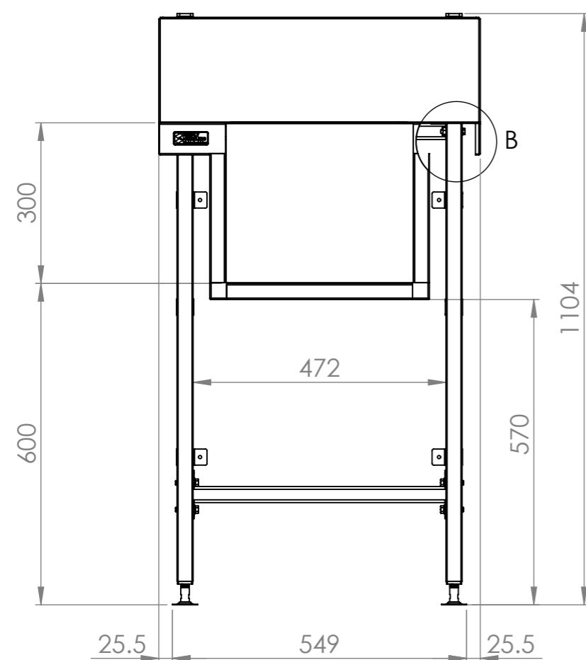
FRONT ELEVATION
