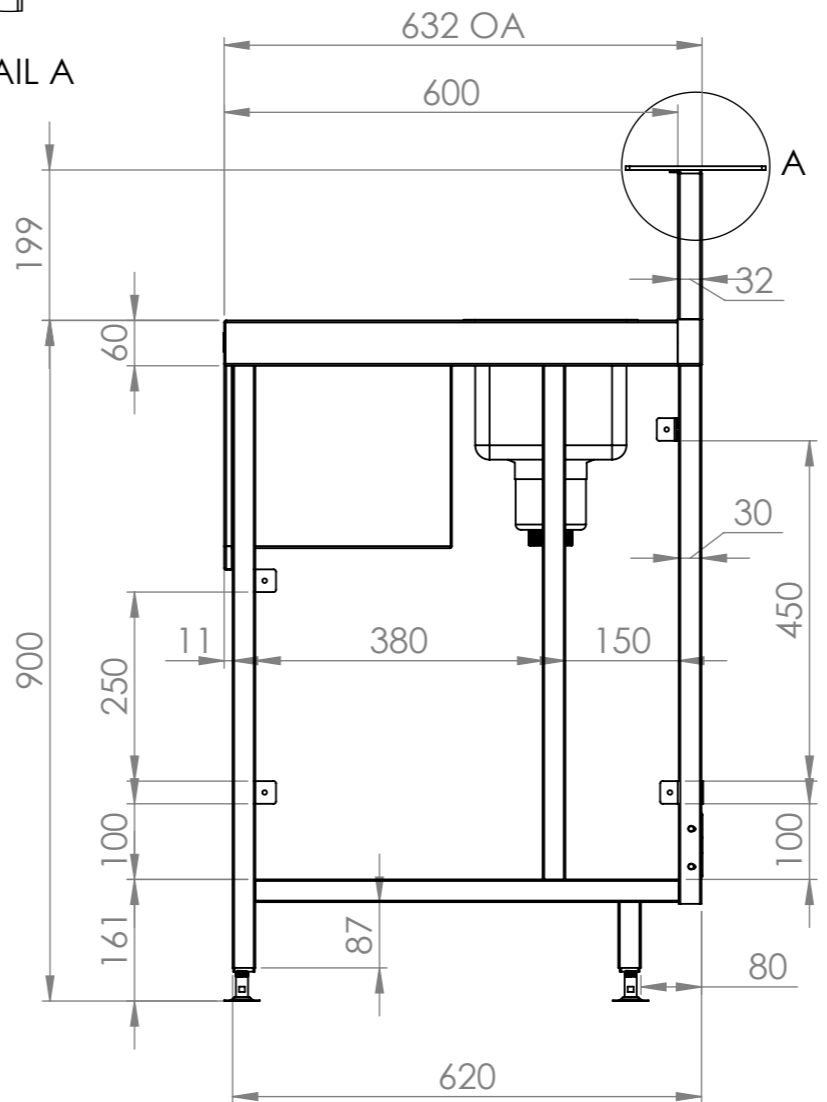
SIDE ELEVATION
