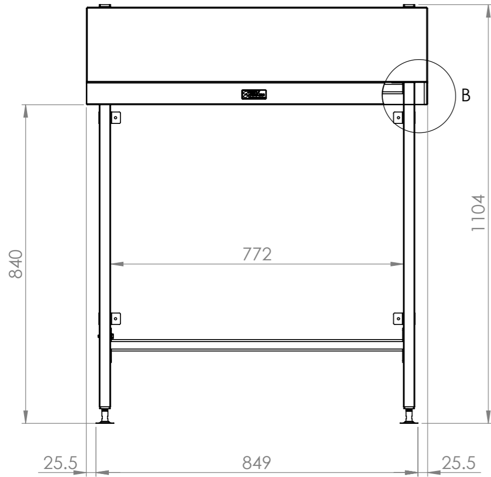
FRONT ELEVATION
