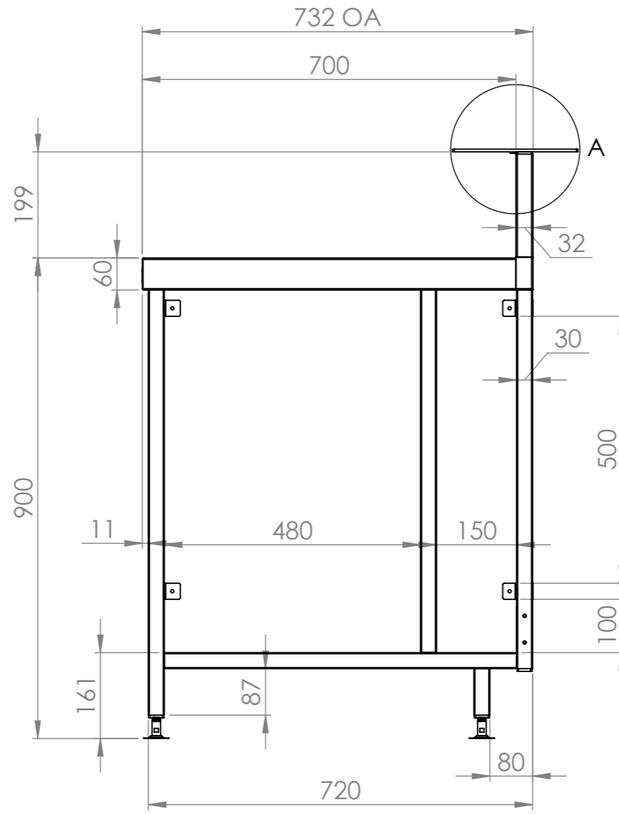
SIDE ELEVATION
