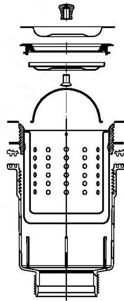
SECTION VIEW
