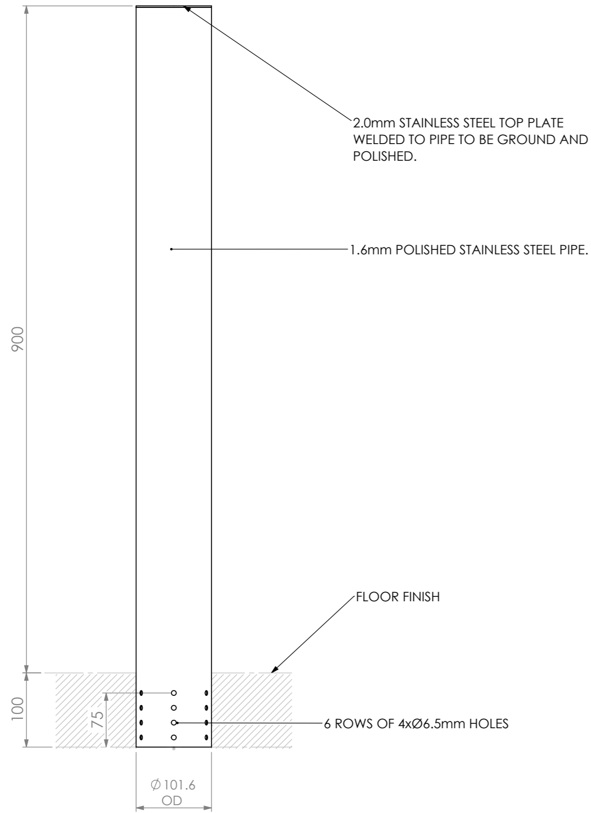
BOLLARD DETAIL SECTION THROUGH
