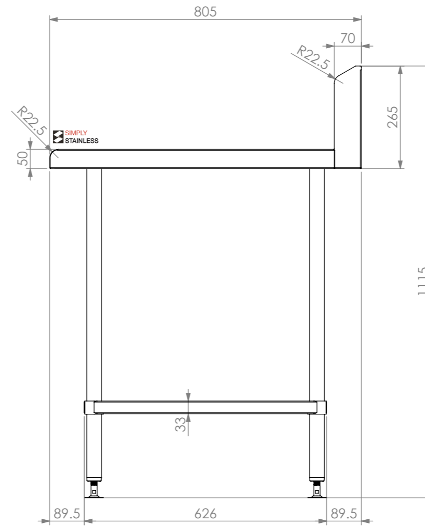
SIDE ELEVATION
