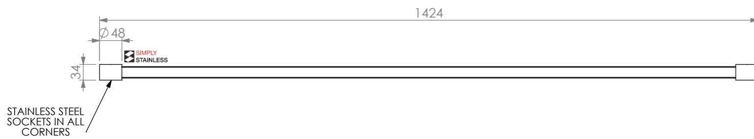
FRONT ELEVATION
