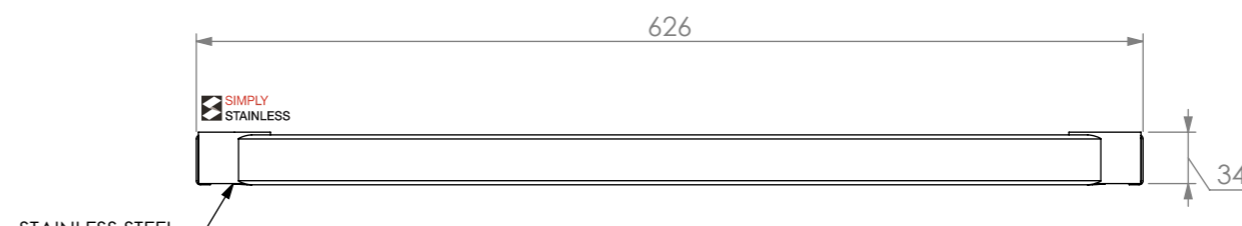
SIDE ELEVATION
