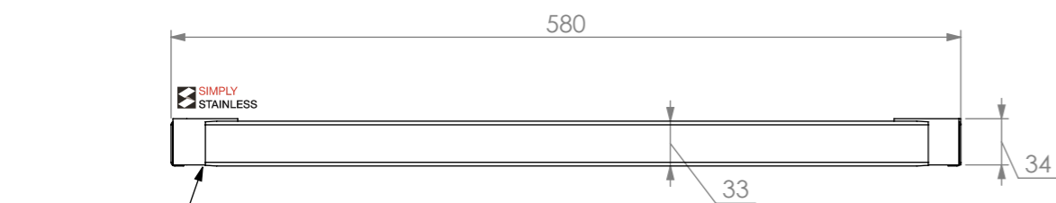
FRONT ELEVATION
