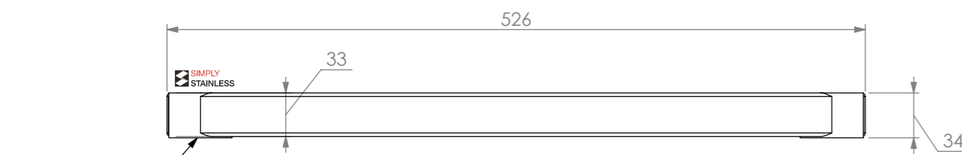
FRONT ELEVATION
