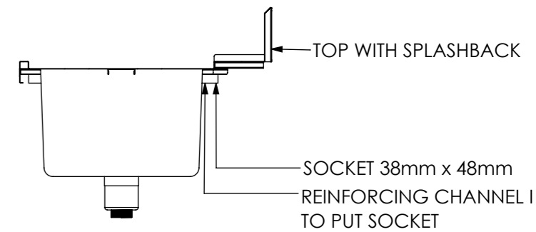
SECTION J-J
