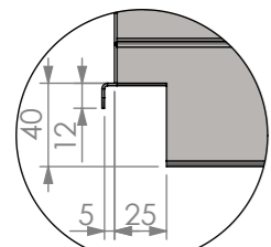
NOTCH DETAIL
