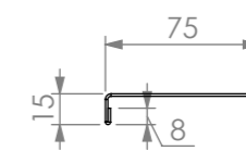
REINFORCING CHANNEL I DETAIL
