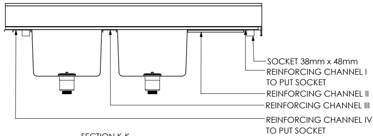
SECTION K-K
