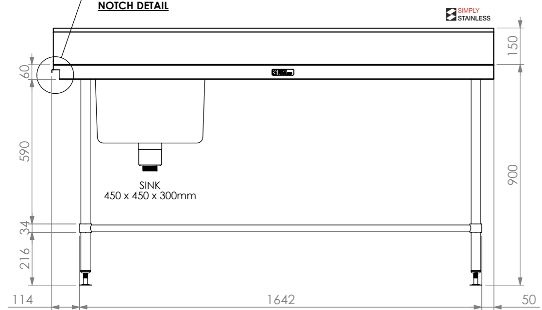
FRONT ELEVATION
