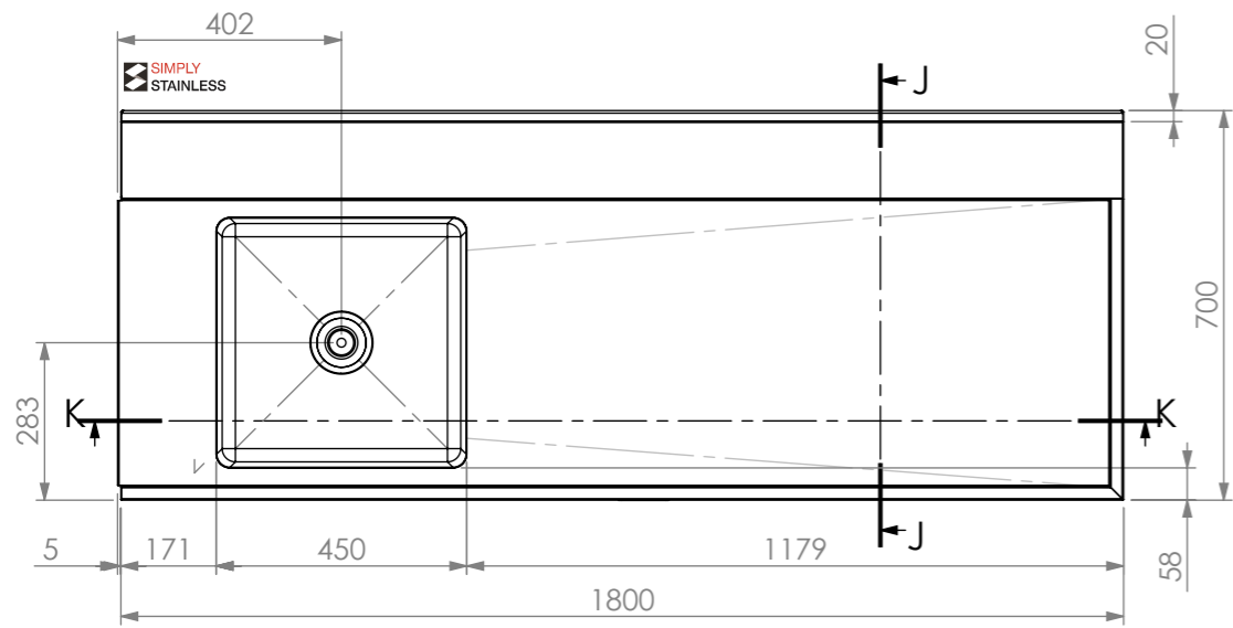
PLAN
