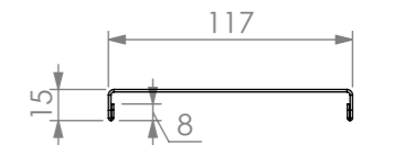
REINFORCING CHANNEL III DETAIL
