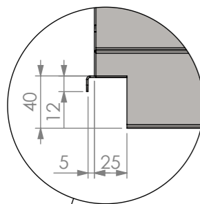
NOTCH DETAIL
