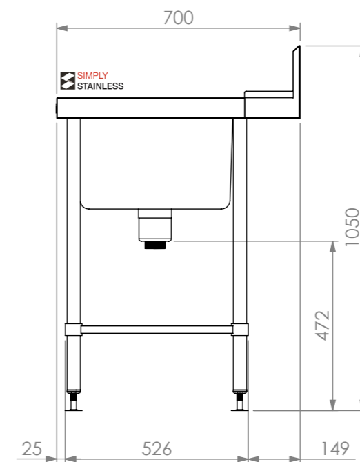
SIDE ELEVATION
