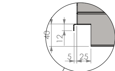
NOTCH DETAIL
