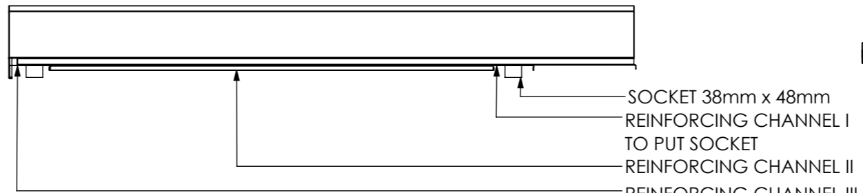
SECTION K-K
