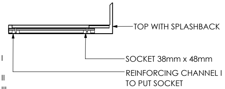
SECTION J-J
