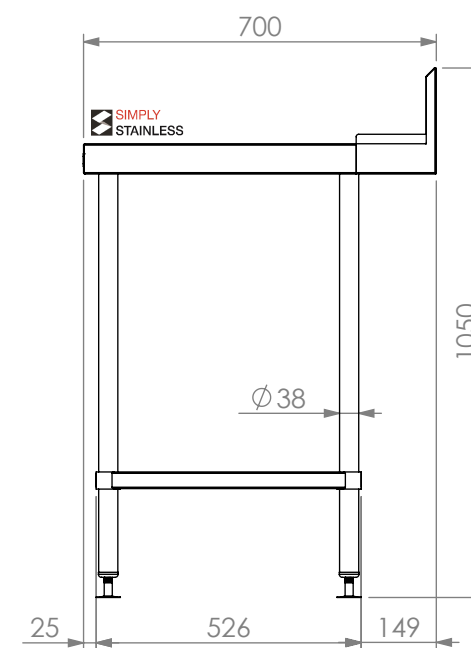
SIDE ELEVATION
