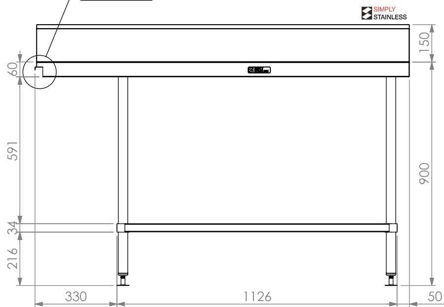
NOTCH DETAIL
