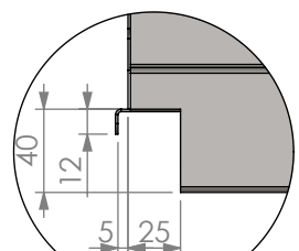
NOTCH DETAIL
