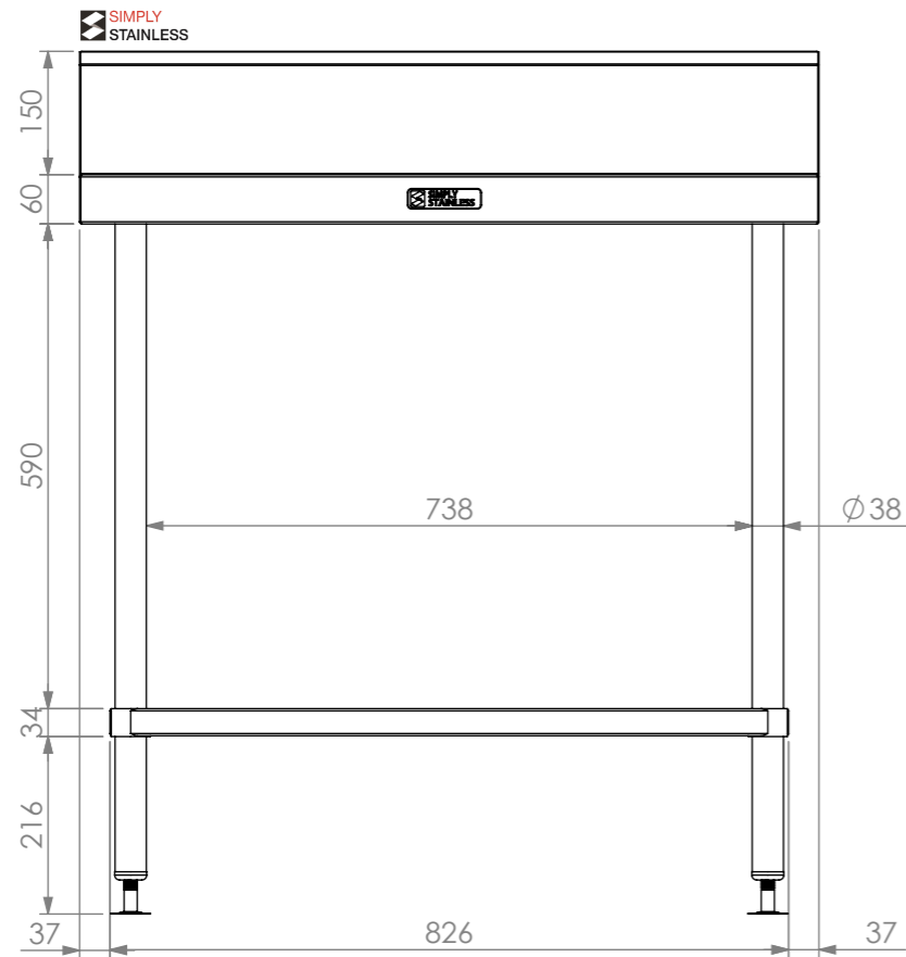
FRONT ELEVATION
