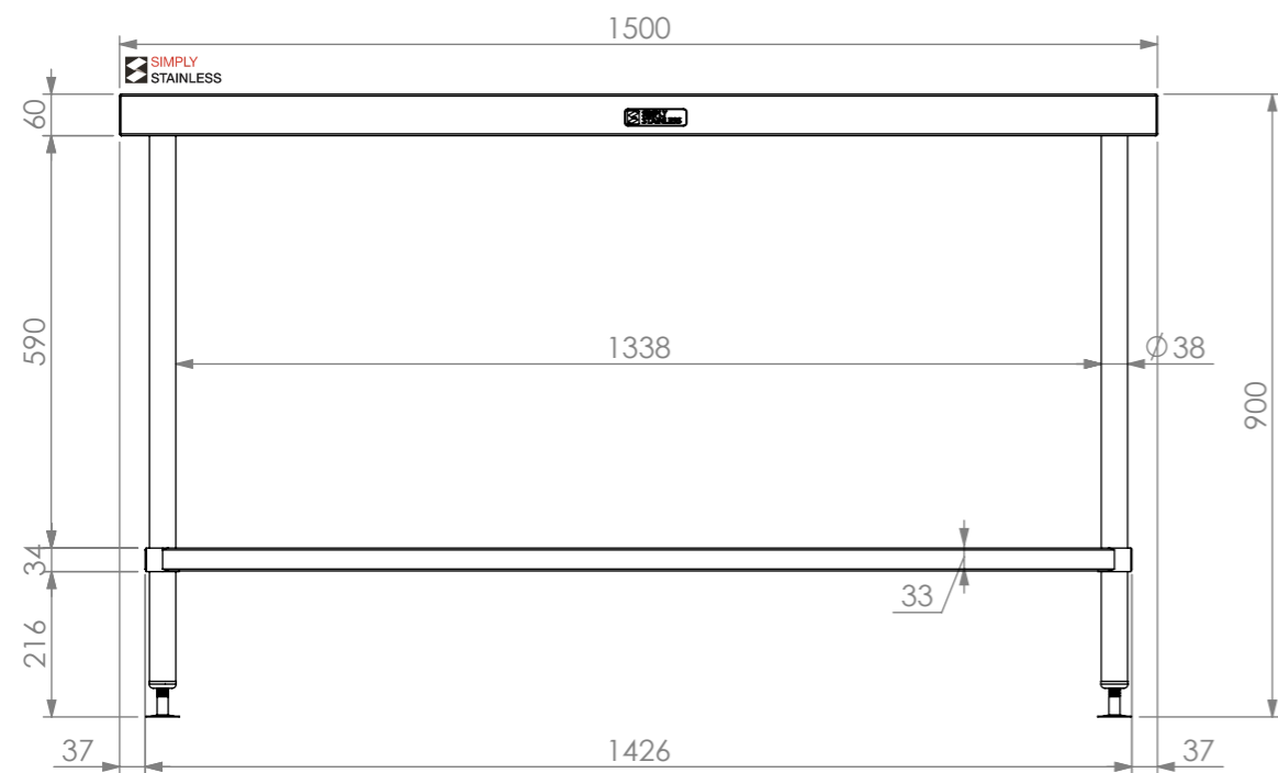
FRONT ELEVATION
