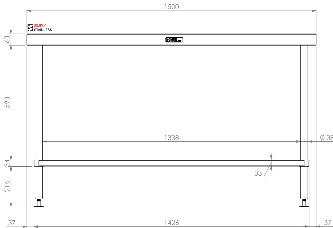
FRONT ELEVATION
