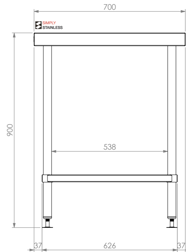
SIDE ELEVATION
