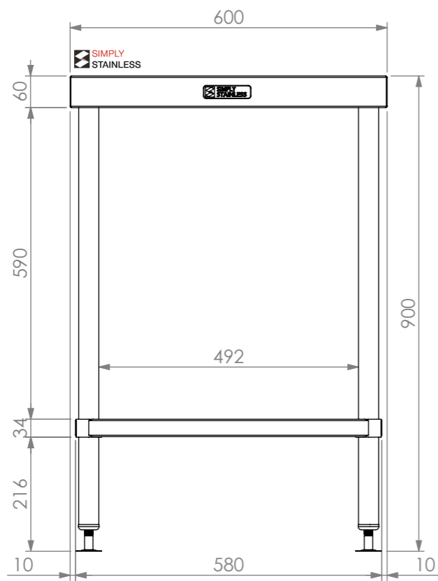
FRONT ELEVATION
