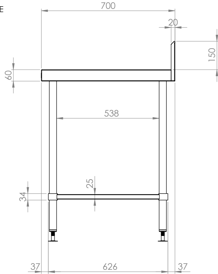
SIDE ELEVATION
