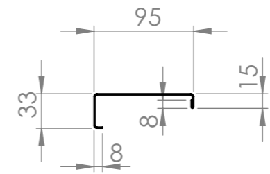
REINFORCING CHANNEL DETAIL
