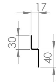
FIXING LUG DETAIL
